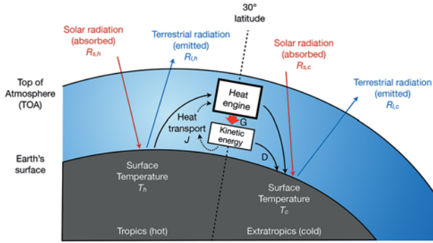
Figure 3: The atmospheric heat engine generates the kinetic energy (wide red arrow, with label G ) associated with large-scale motion from the heat it transports from the tropics to the extratropics to balance out differences in absorbed solar radiation. The generated kinetic energy sustains the atmospheric motion that accomplishes the heat transport, as indicated by the dotted arrows. The different symbols next to the terms are used for the estimate described in the text.
