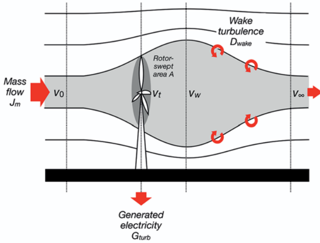
Figure A.1: Schematic diagram of a wind turbine and the surrounding mass flow, with different wind velocities of the unaffected flow ( v_0 ), at the turbine ( v_t ), within the wake ( v_w ) and after the wake was dissolved by wake turbulence ( v_\infty ).
